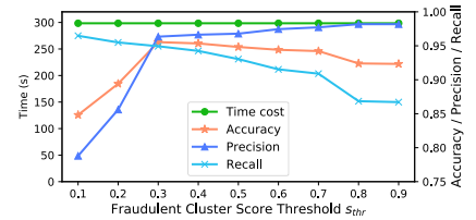
Figure 15: s_{thr} Experiment
