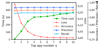
Figure 13: \eta Experiment
