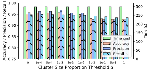
Figure 16: \alpha Experiment
