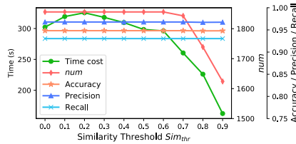
Figure 14: Sim_{thr} Experiment
