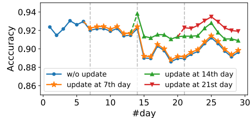
Figure 17: Accuracy with and without updating.
