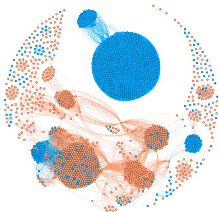
Figure 5: A sample device graph constructed by 1,000 fraudulent vertices (in blue) and 1,000 benign vertices (in orange).
