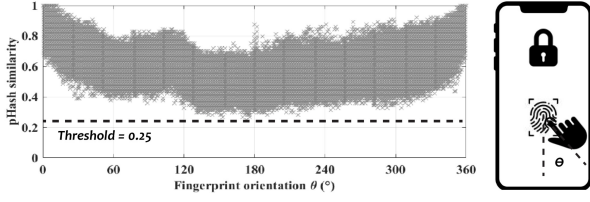
Fig. 19: pHash similarities with different fingerprint orientations ( 0^\circ – 360^\circ ) that are recognizable to the in-display fingerprint sensor.
