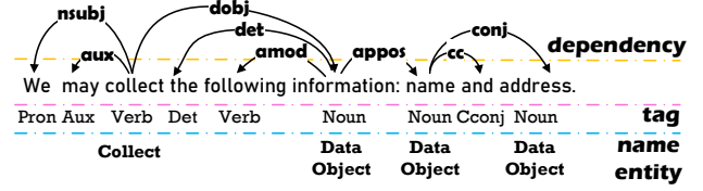
Figure 1: Sentence parsing
